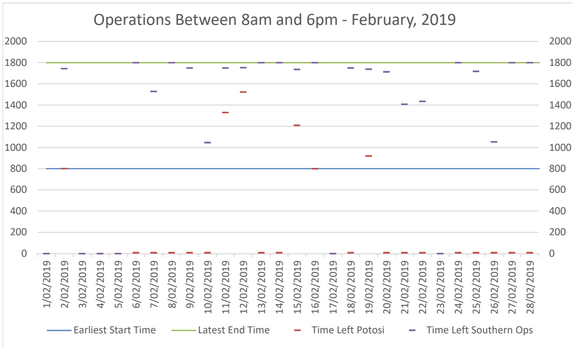
Graph 1 - Haulage Times
