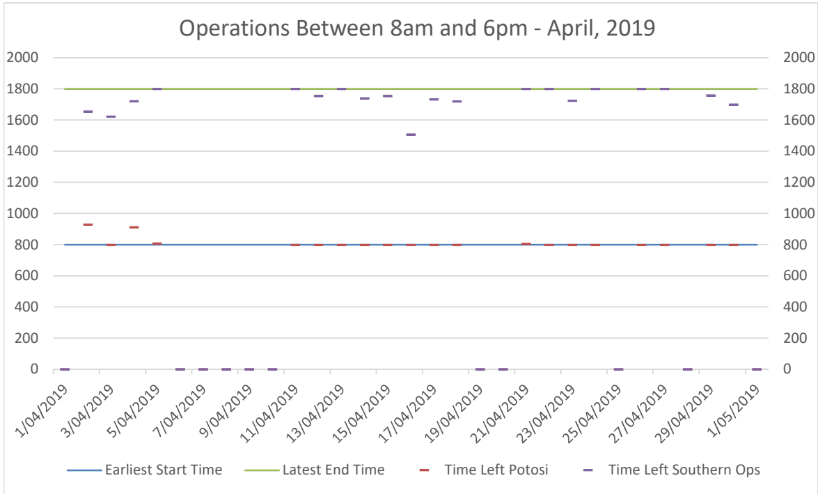
Graph 1 - Haulage Times
