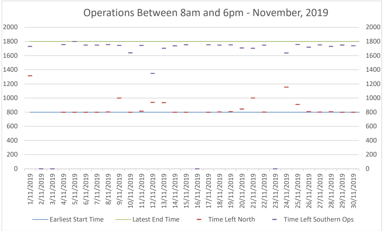
Graph 1 - Haulage Times
