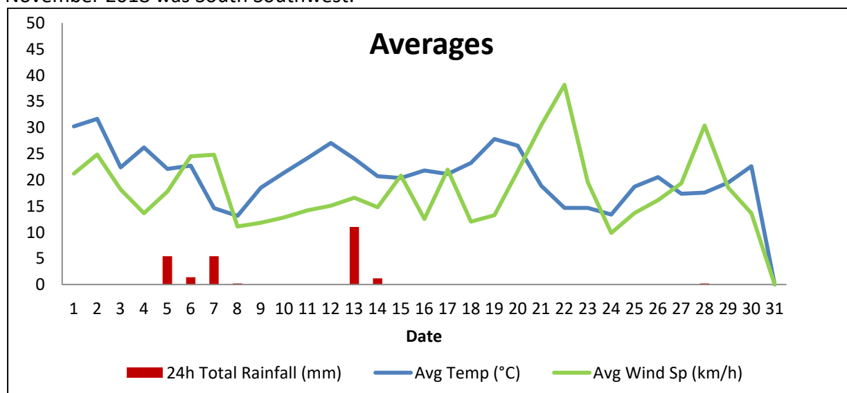
Figure 1. Average wind speed (km/hr) and daily rainfall (mm) for November 2018.
