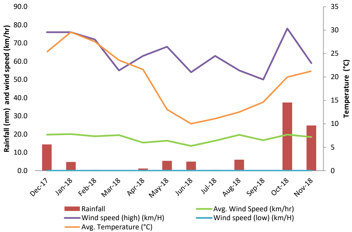
Figure 2. Average monthly temperature, wind speed and total rainfall for the 12 months up to and including November 2018.
