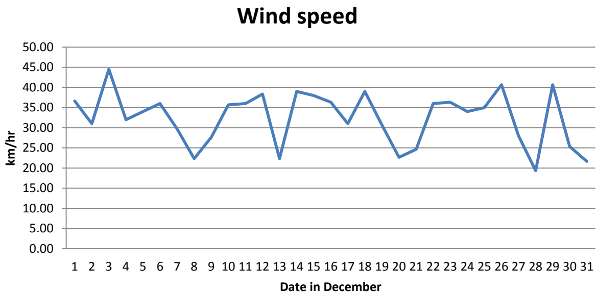
Figure 1. Average wind speed (km/hr) on a daily basis for December 2014.
