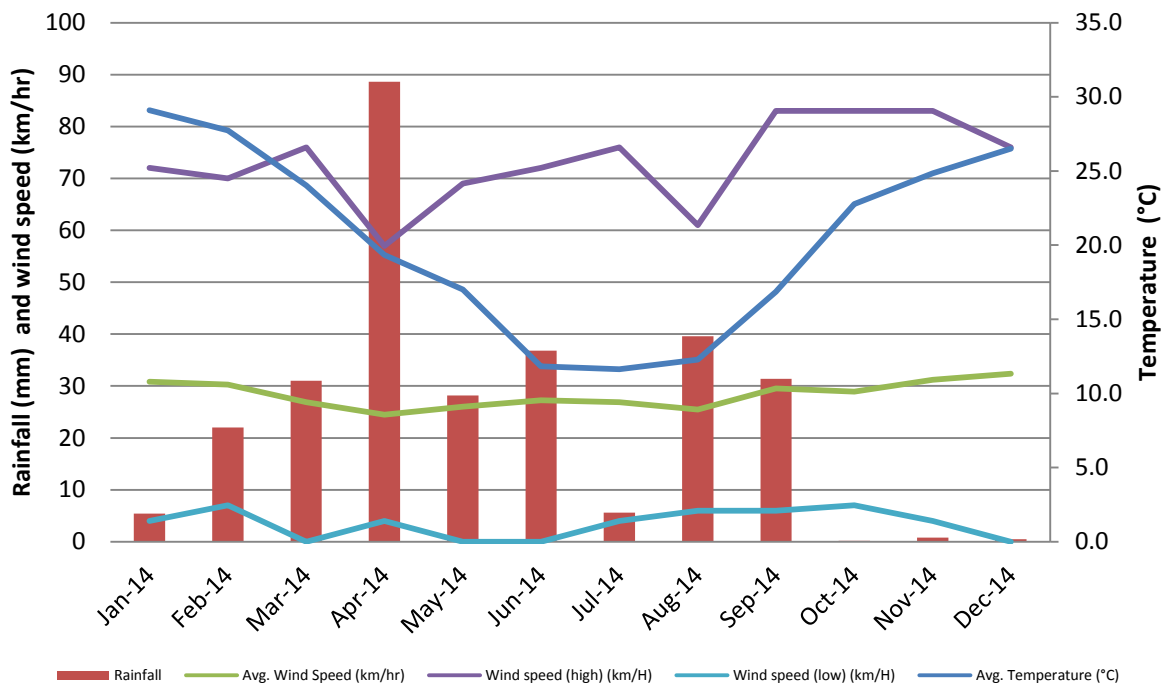
Figure 2. Average monthly temperature, wind speed and total rainfall for the 12 months up to and including December 2014.
