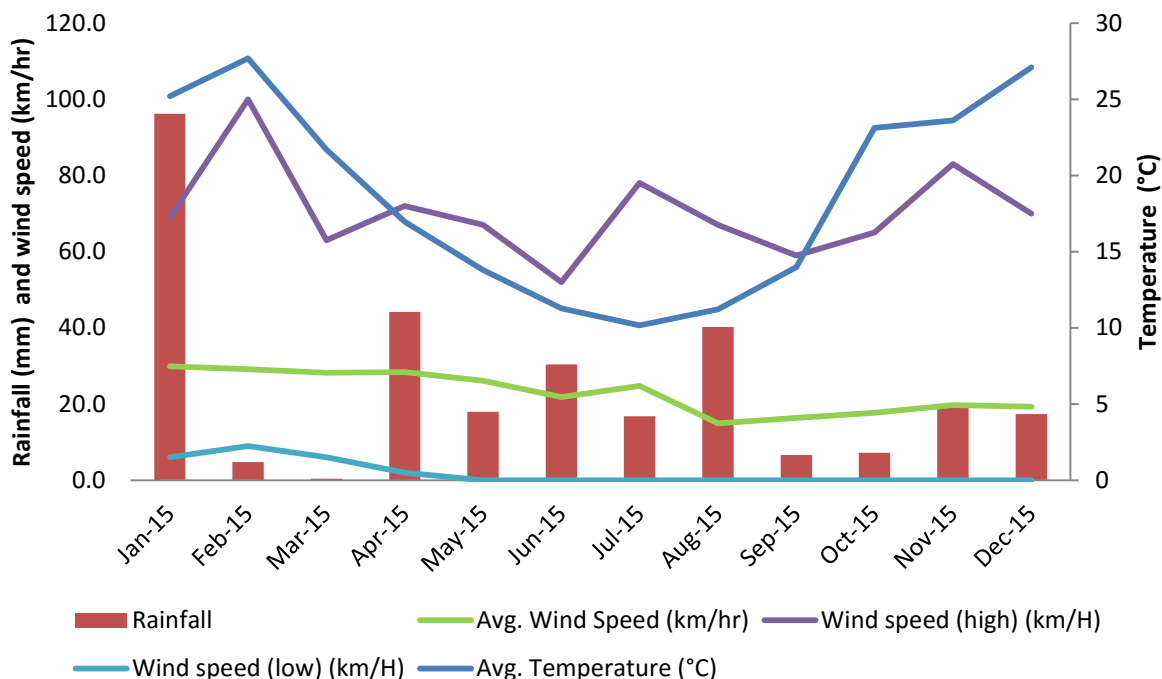
Figure 2. Average monthly temperature, wind speed and total rainfall for the 12 months up to and including December 2015.
