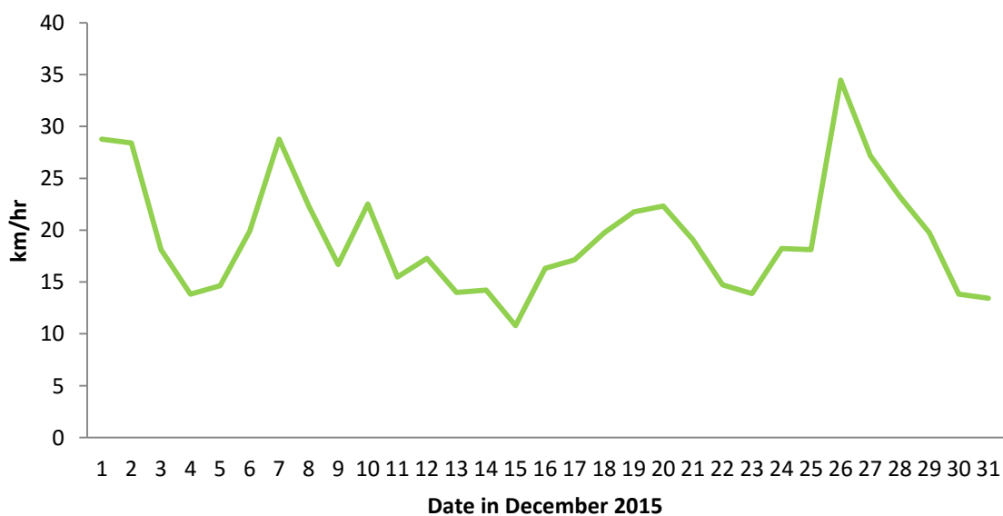
Figure 1. Average wind speed (km/hr) on a daily basis for December 2015.
