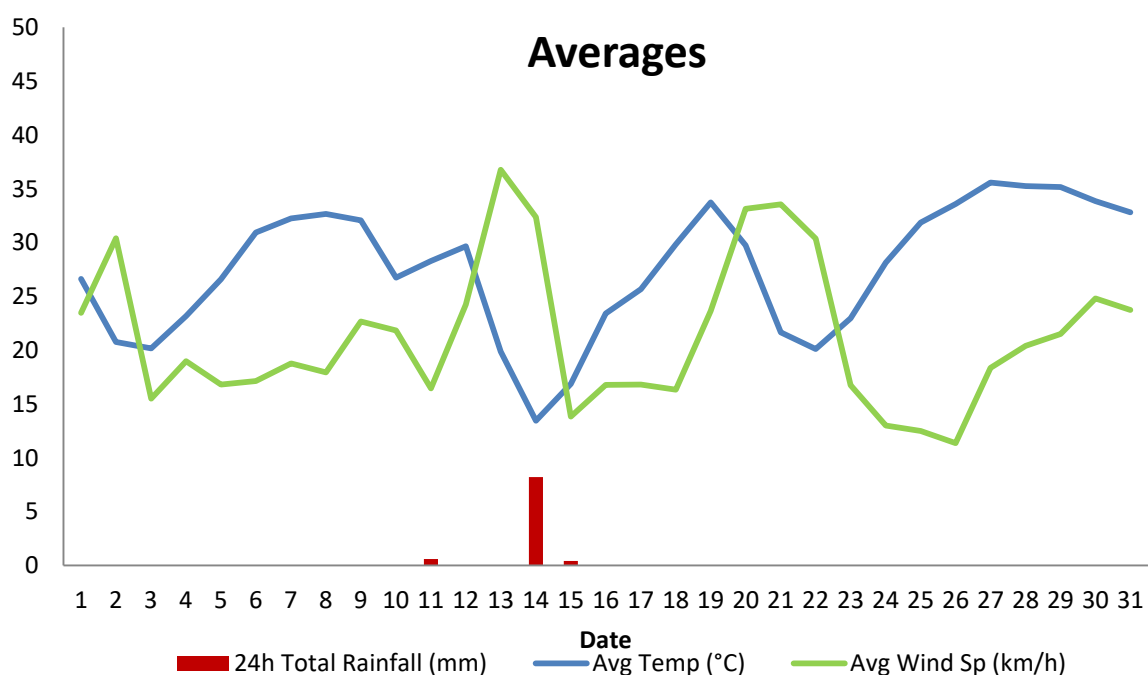
Figure 1. Average wind speed (km/hr) and daily rainfall (mm) for December 2018.
