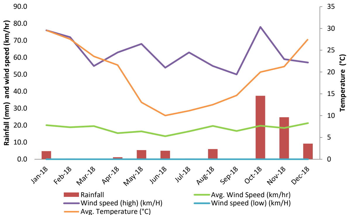
Figure 2. Average monthly temperature, wind speed and total rainfall for the 12 months up to and including December 2018.
