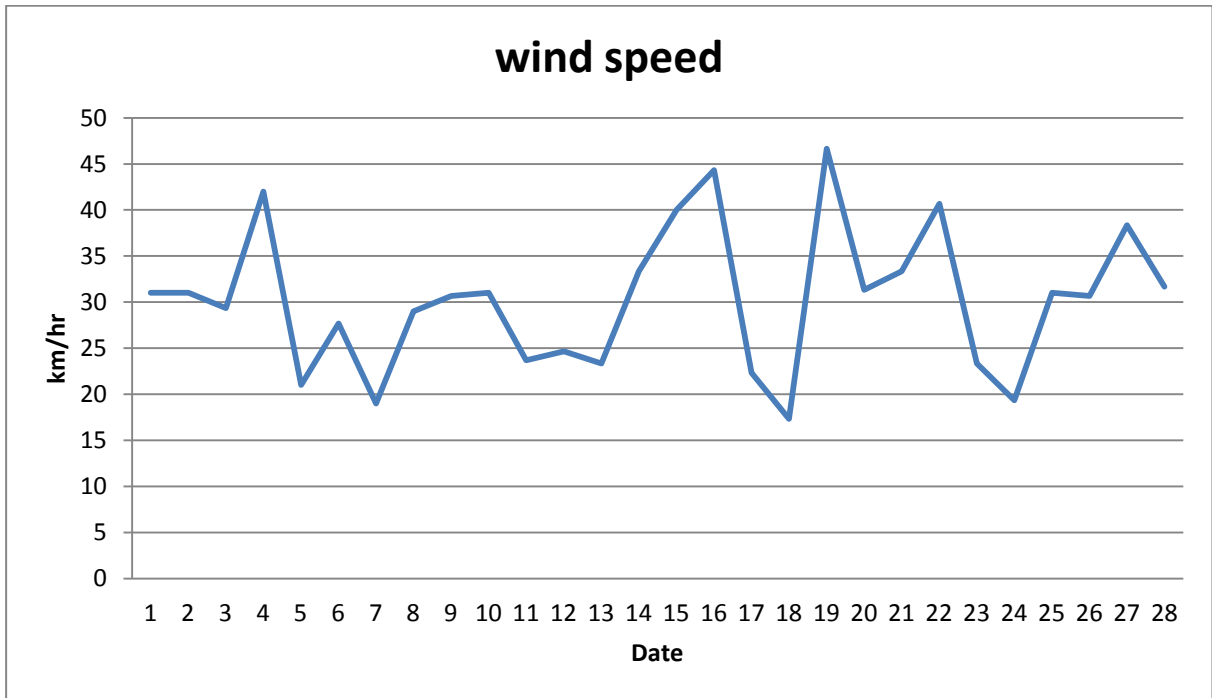
Figure 1. Average wind speed (km/hr) on a daily basis for February.
