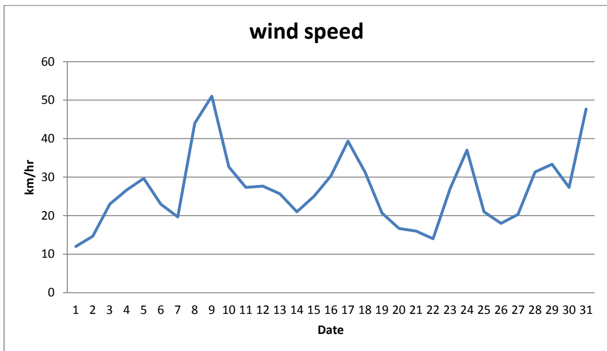
Figure 1. Average wind speed (km/hr) on a daily basis for July.
