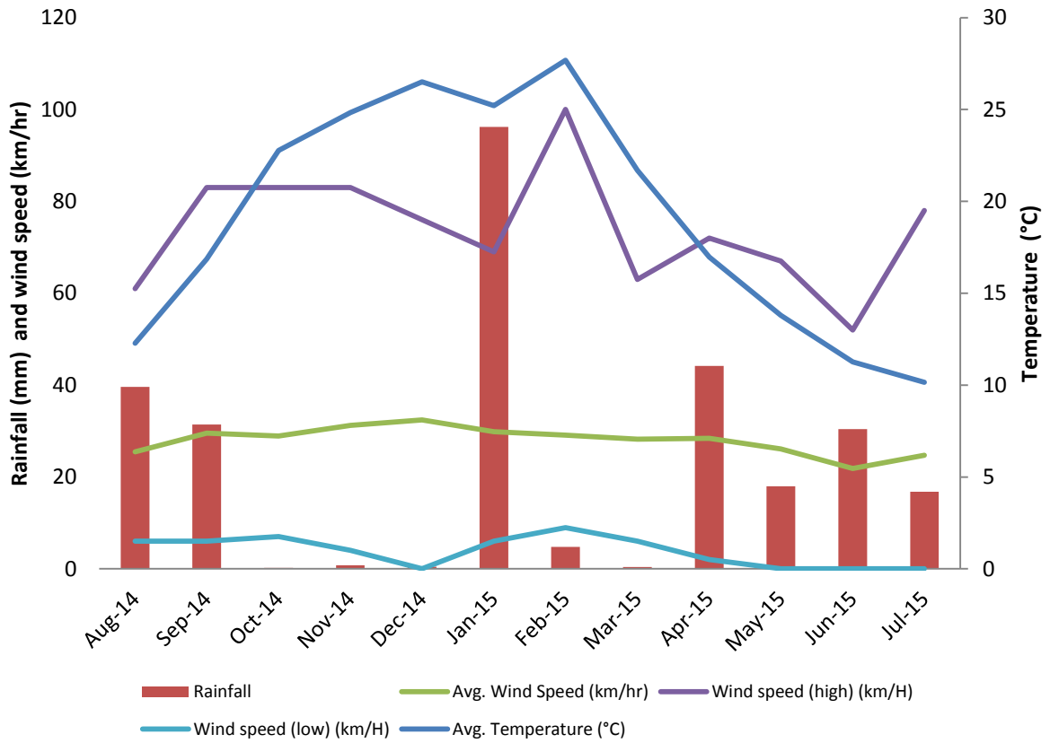
Figure 2. Average monthly temperature, wind speed and total rainfall for the 12 months up to and including July 2015.
