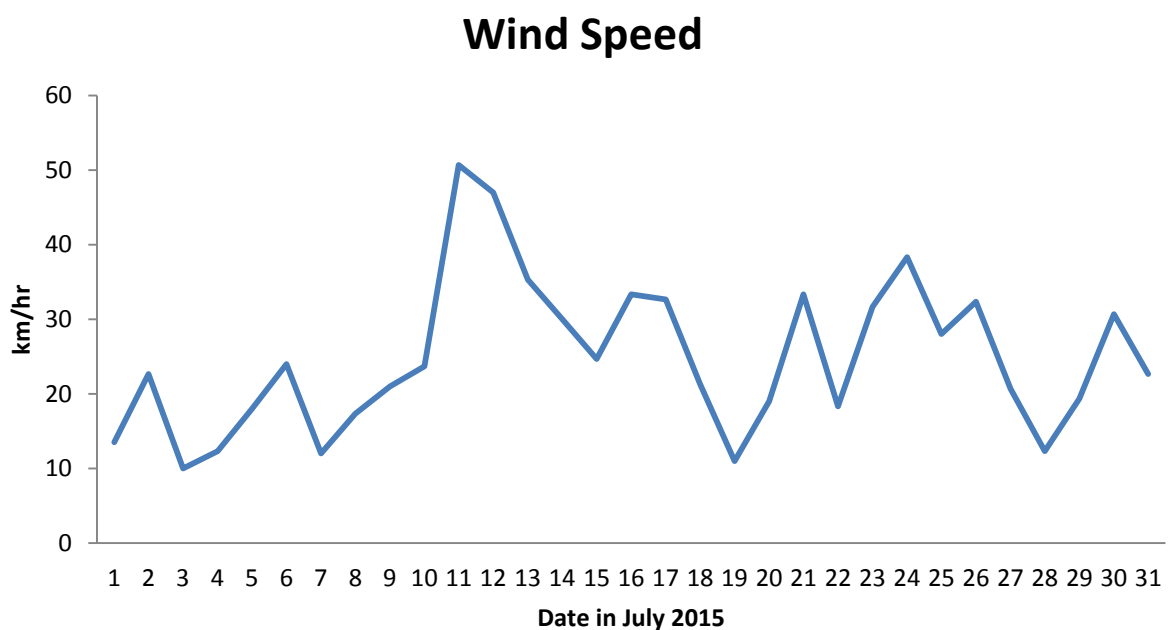
Figure 1. Average wind speed (km/hr) on a daily basis for July 2015.
