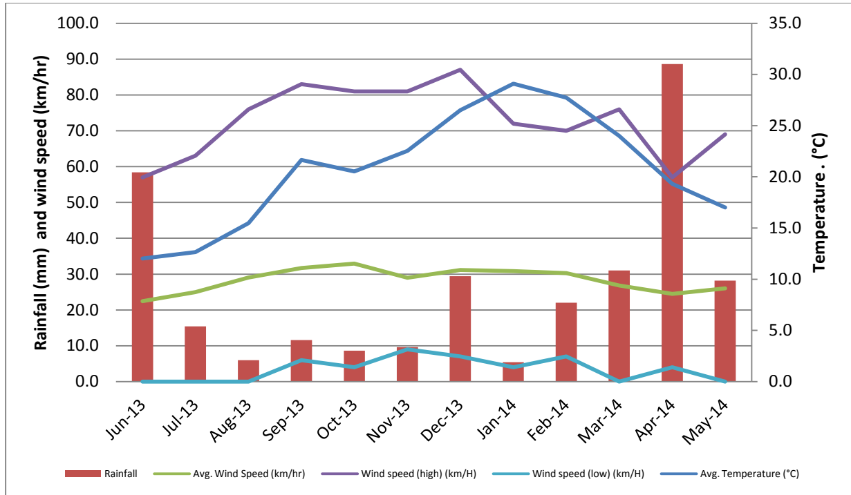
Figure 2. Average monthly temperature, wind speed and total rainfall for the previous 12 months.
