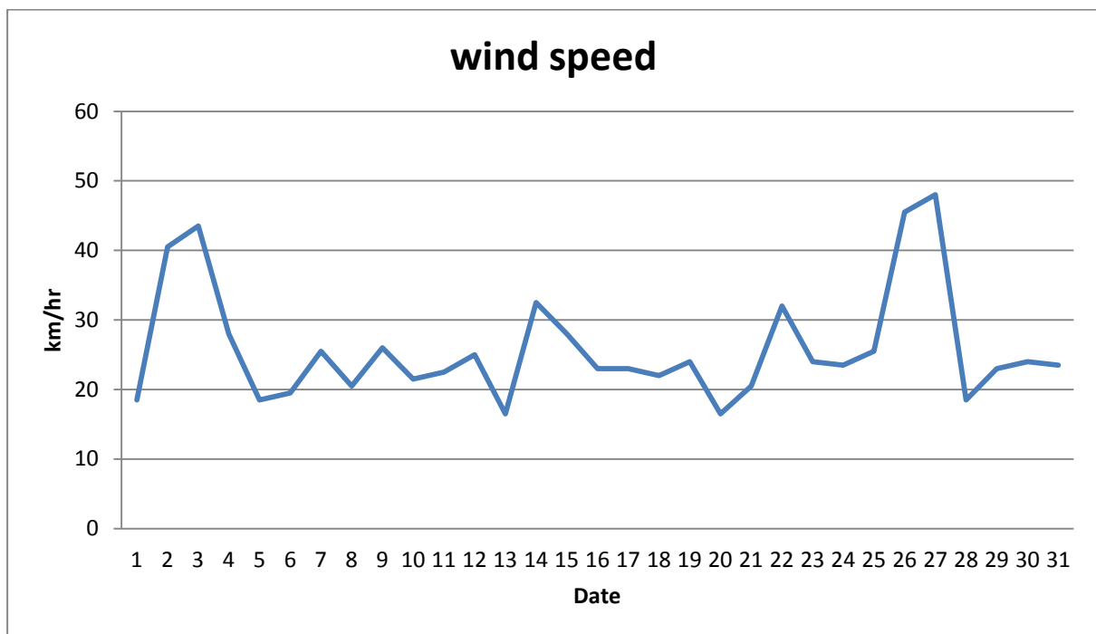
Figure 1. Average wind speed (km/hr) on a daily basis for May.
