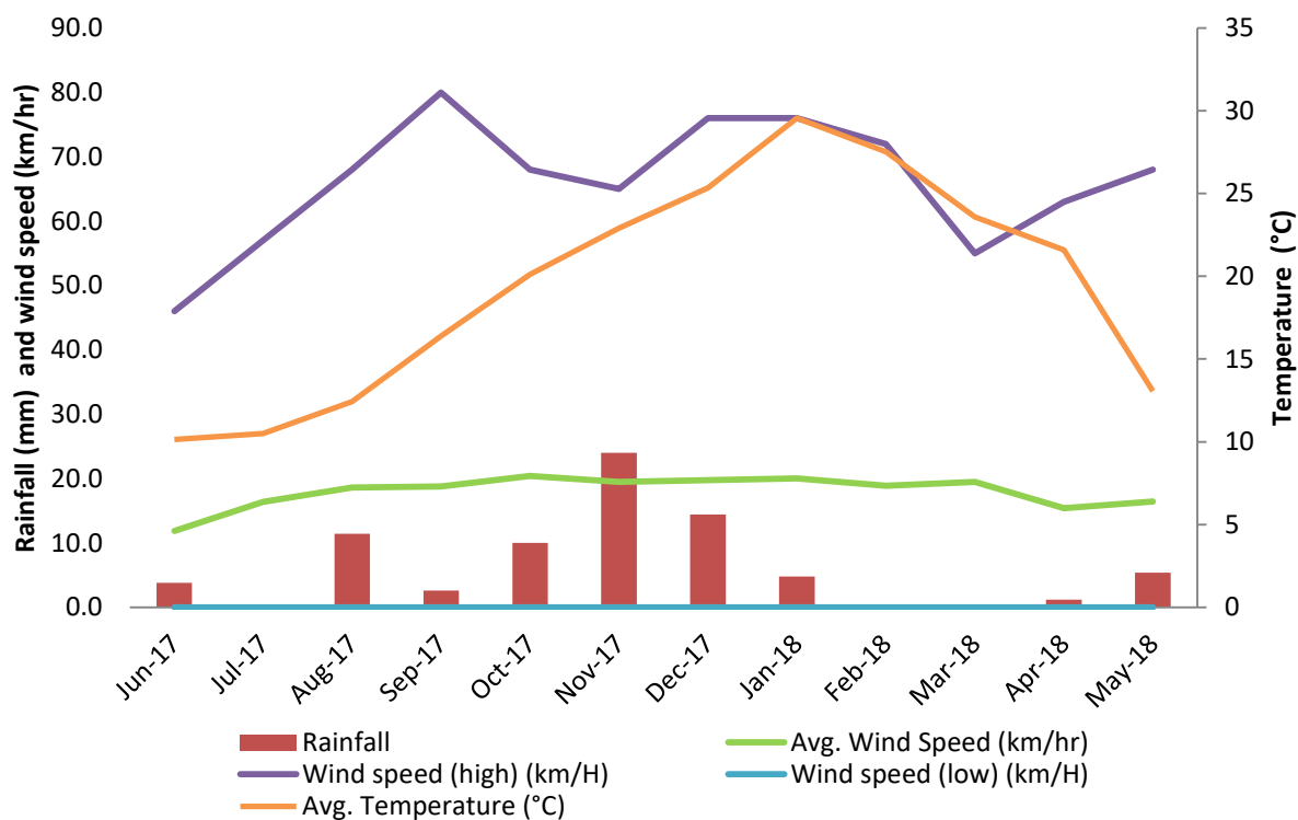
Figure 2. Average monthly temperature, wind speed and total rainfall for the 12 months up to and including May 2018.
