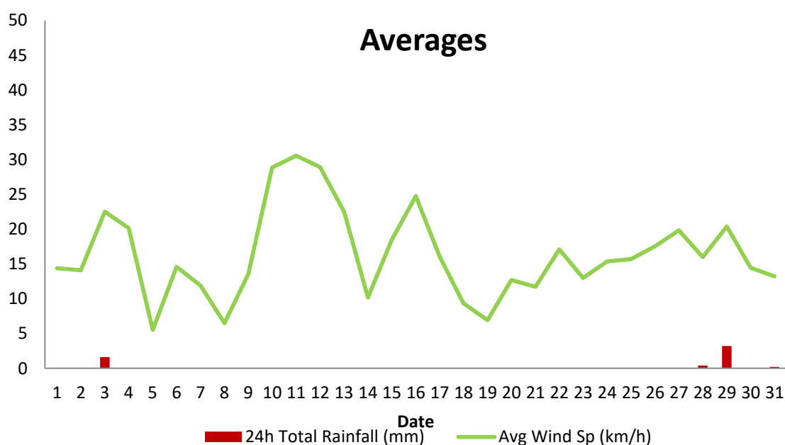
Figure 1. Average wind speed (km/hr) and daily rainfall (mm) for May 2018.
