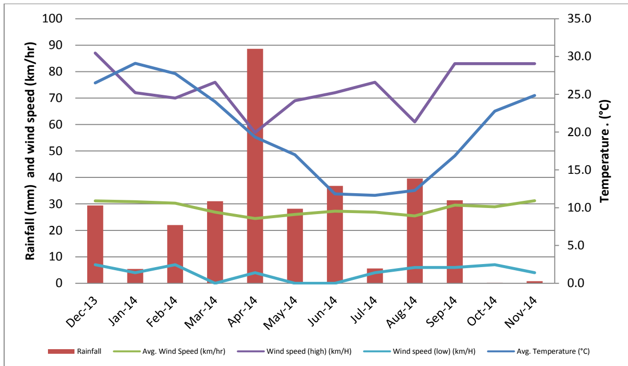
Figure 2. Average monthly temperature, wind speed and total rainfall for the 12 months up to and including November 2014.
