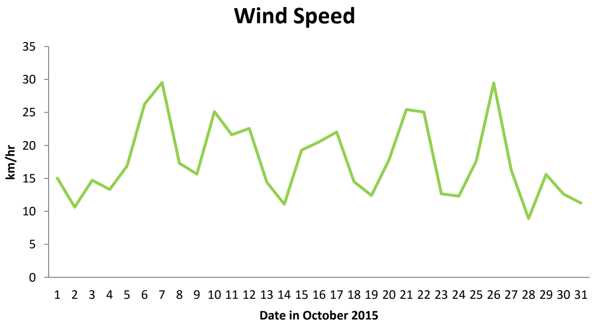
Figure 1. Average wind speed (km/hr) on a daily basis for October 2015.
