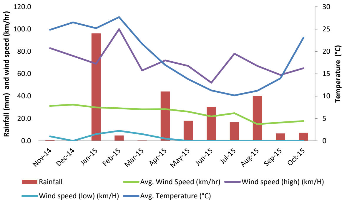
Figure 2. Average monthly temperature, wind speed and total rainfall for the 12 months up to and including October 2015.
