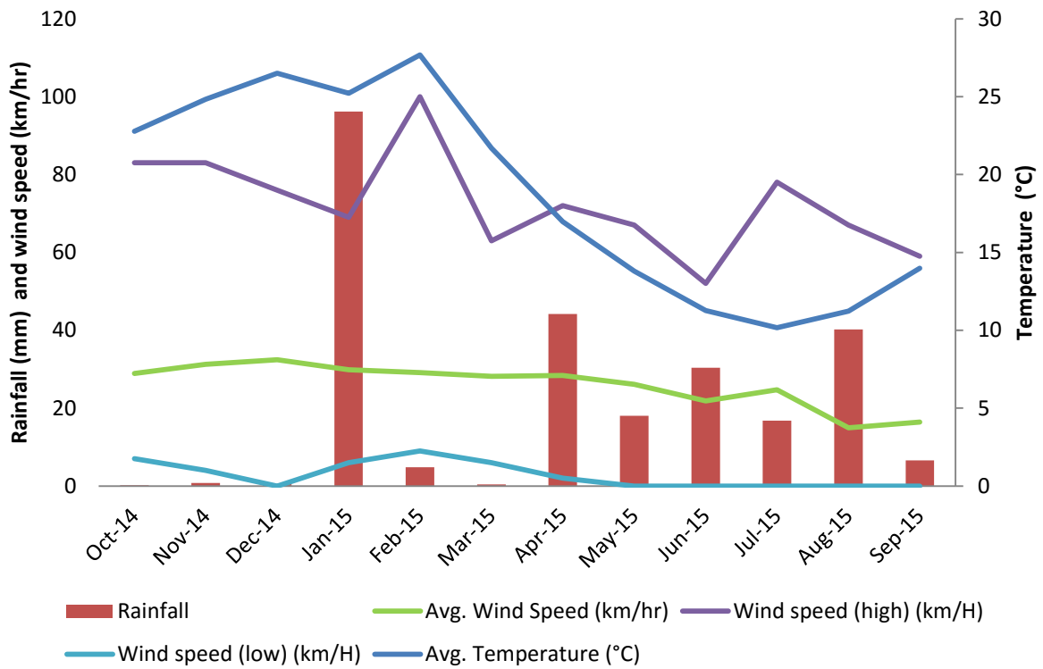
Figure 2. Average monthly temperature, wind speed and total rainfall for the 12 months up to and including September 2015.
