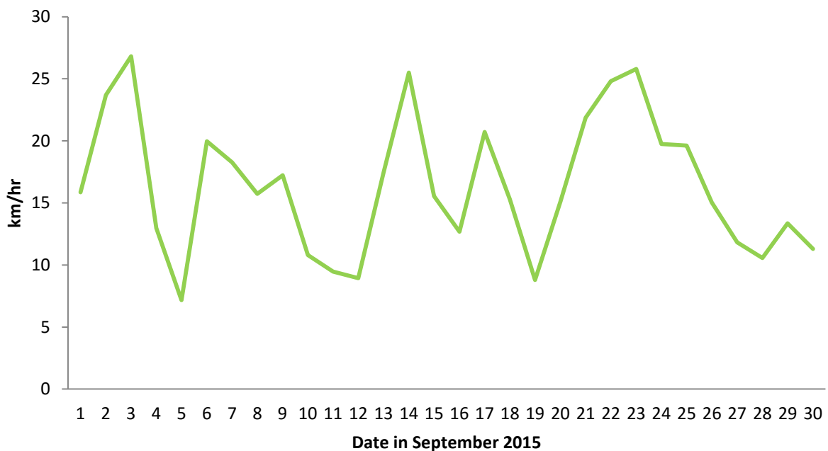
Figure 1. Average wind speed (km/hr) on a daily basis for September 2015.
