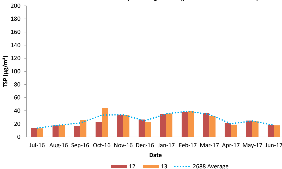
Figure 3. Average TSP results for the 12 months up to and including June.
