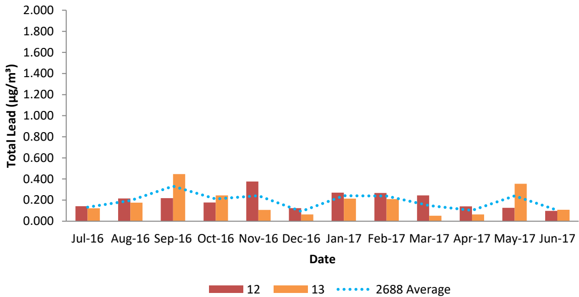
Figure 4. Average total lead results for the 12 months up to and including June.
