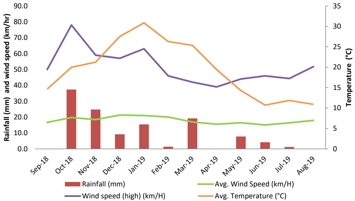
Figure 2. Average monthly temperature, wind speed and total rainfall for the 12 months up to and including August 2019.
