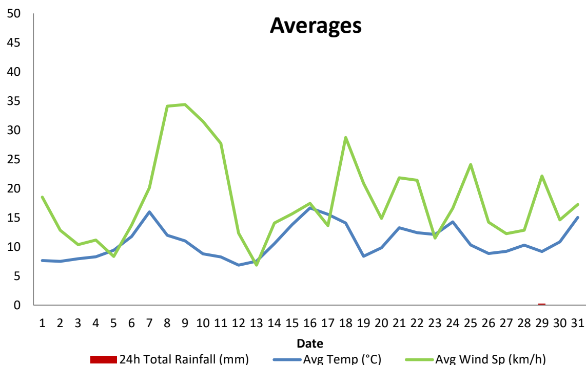
Figure 1. Average wind speed (km/hr) and daily rainfall (mm) for August 2019.
