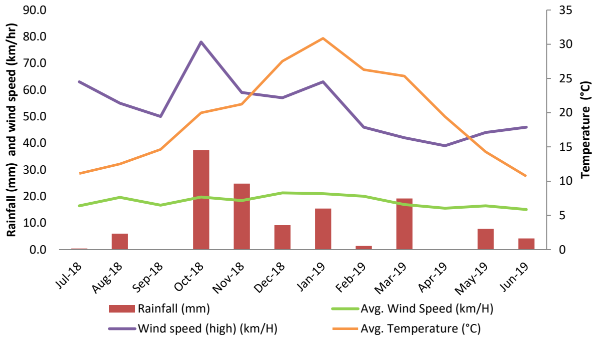
Figure 2. Average monthly temperature, wind speed and total rainfall for the 12 months up to and including June 2019.
