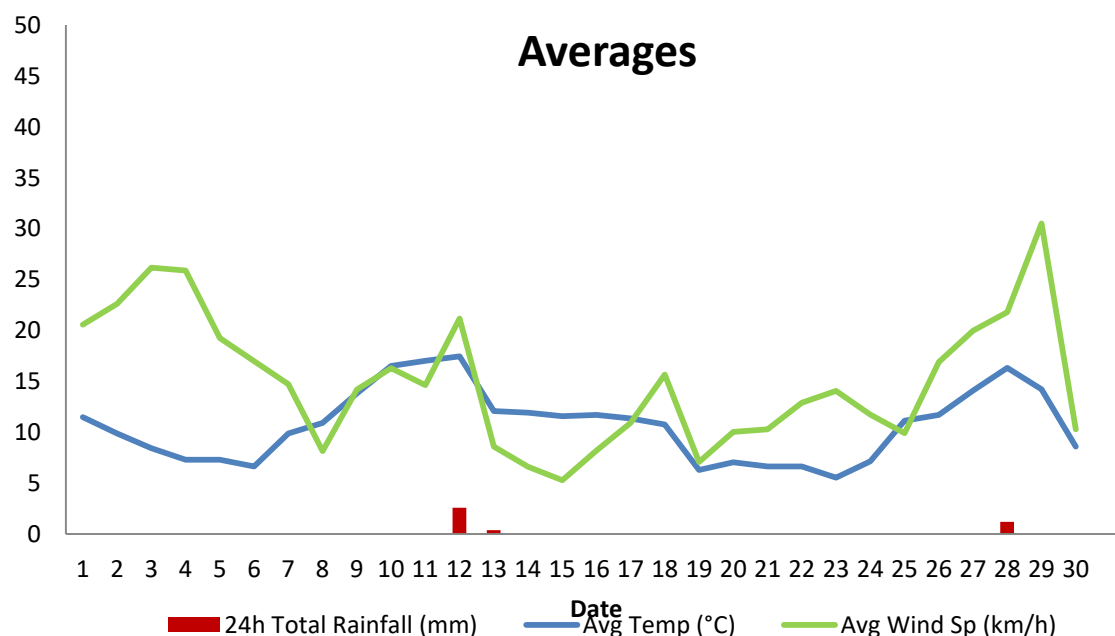
Figure 1. Average wind speed (km/hr) and daily rainfall (mm) for June 2019.
