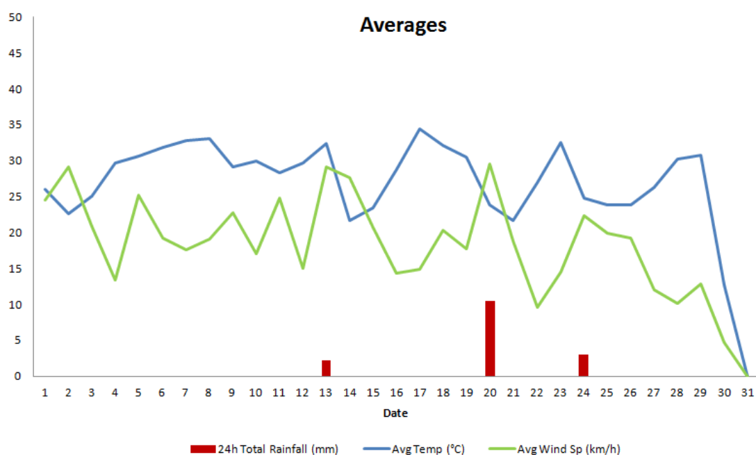
Figure 1. Average wind speed (km/hr) and daily rainfall (mm) for January 2017.
