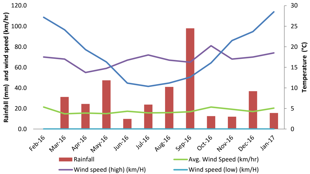
Figure 2. Average monthly temperature, wind speed and total rainfall for the 12 months up to and including January 2017.
