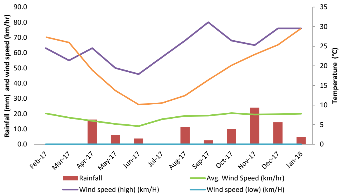
Figure 2. Average monthly temperature, wind speed and total rainfall for the 12 months up to and including January 2018.
