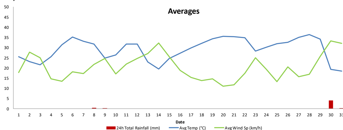
Figure 1. Average wind speed (km/hr) and daily rainfall (mm) for January 2018.
