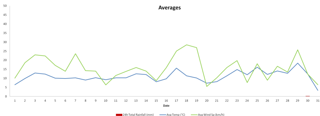
Figure 1. Average wind speed (km/hr) and daily rainfall (mm) for July 2017.
