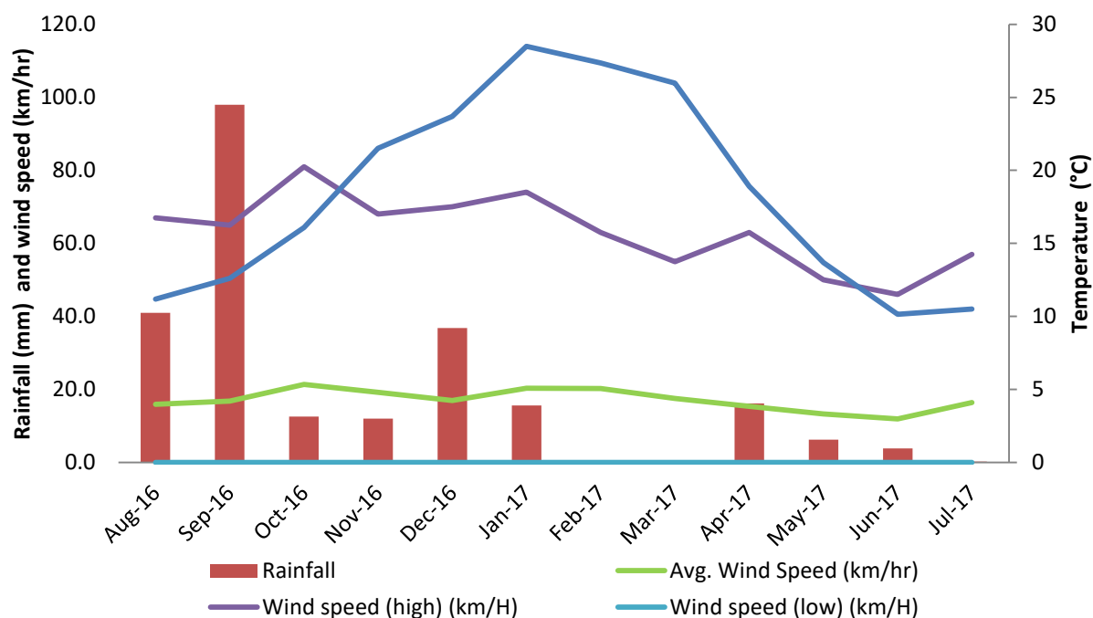
Figure 2. Average monthly temperature, wind speed and total rainfall for the 12 months up to and including July 2017.
