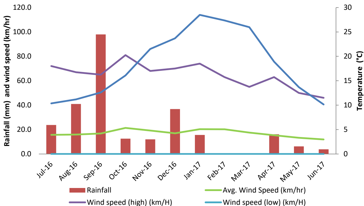
Figure 2. Average monthly temperature, wind speed and total rainfall for the 12 months up to and including June 2017.
