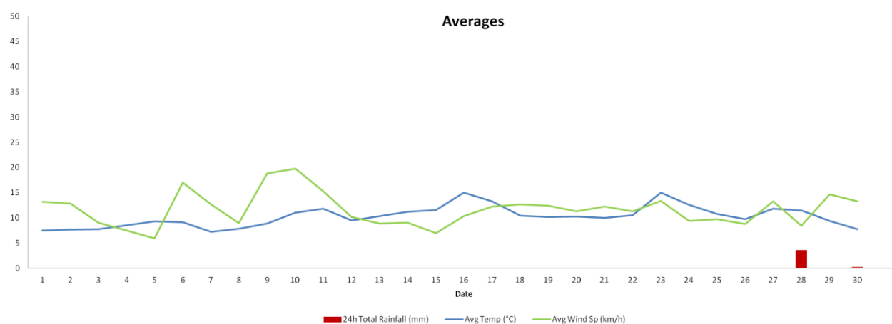
Figure 1. Average wind speed (km/hr) and daily rainfall (mm) for June 2017.
