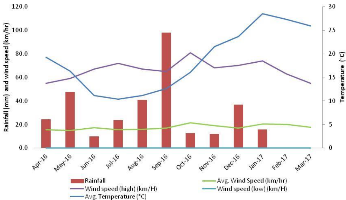
Figure 2. Average monthly temperature, wind speed and total rainfall for the 12 months up to and including March 2017.
