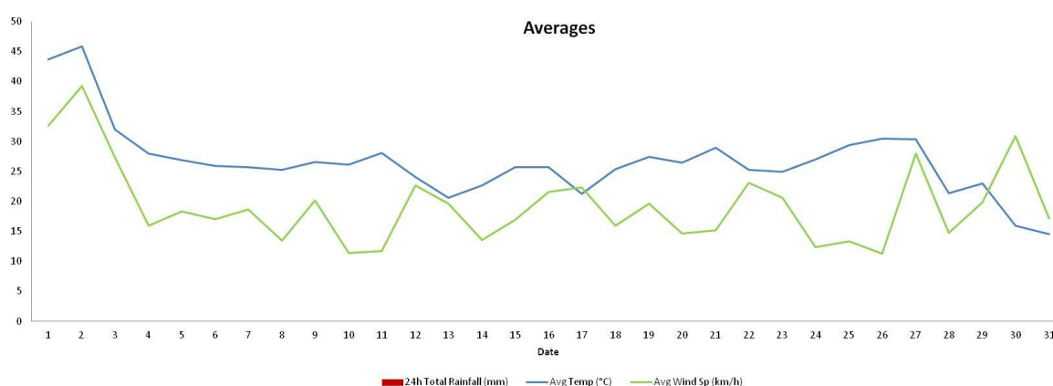
Figure 1. Average wind speed (km/hr) and daily rainfall (mm) for March 2017.
