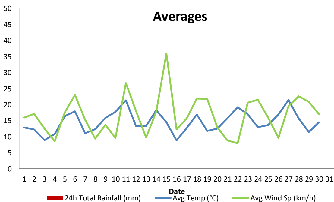
Figure 1. Average wind speed (km/hr) and daily rainfall (mm) for September 2018.
