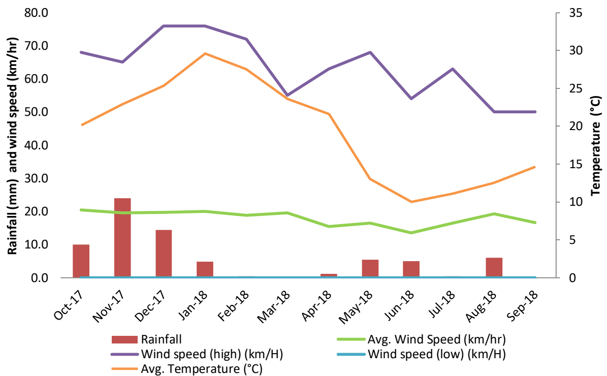
Figure 2. Average monthly temperature, wind speed and total rainfall for the 12 months up to and including September 2018.
